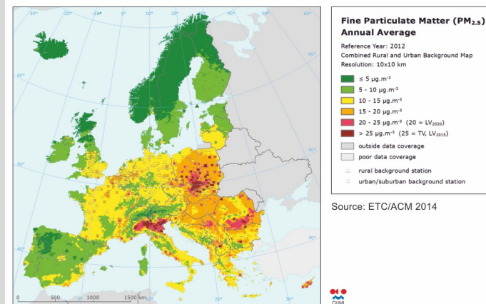
Fig. VIII.3 Annual average concentration of PM 2.5 in Europe, 2012
